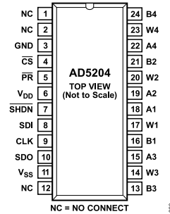
Figure 6. AD5204 SOIC/TSSOP Pin Configuration
